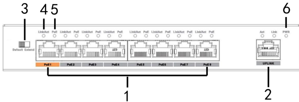
Figure 2-1 Front panel
