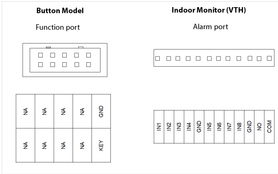
Figure 1-15 Cable connection
