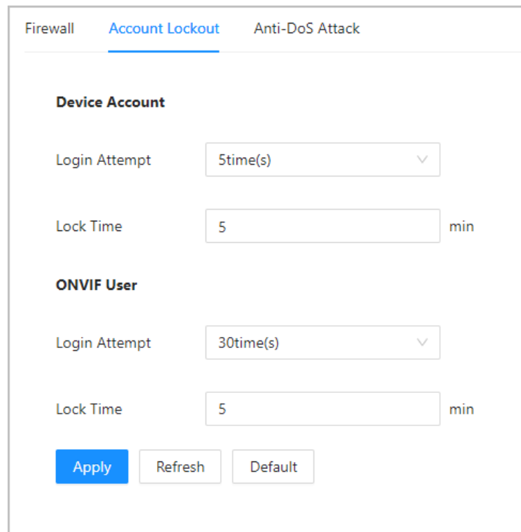
Figure 12-5 Account lockout
