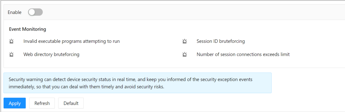
Figure 12-10 Security warning
